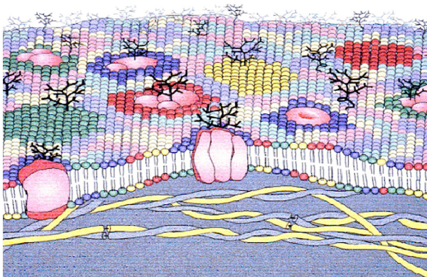
Fig. 4. A schematic illustration of a modification of the Fluid–Mosaic Membrane Model, as envisioned by Escribá and colleagues in 2008. Different lipids are indicated in various colors forming specialized domains around integral membrane proteins and glycoproteins as well as being asymmetrically distributed across the membrane. From Escribá et al. [228].
