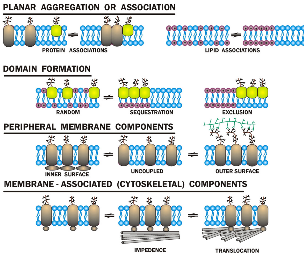
Fig. 3. Some proposed mobility-restraining mechanisms that could potentially affect the rates of lateral diffusion and mobility of membrane glycoproteins and phospholipids in the membrane plane, as envisioned in 1976. In this scheme, different mechanisms (glycoprotein complexes, membrane domains, cytoskeletal interactions, extracellular matrix interactions, peripheral membrane protein interactions, lipid-lipid interactions, etc.) can restrain the lateral movements of membrane components and affect their macromolecular structures and distributions. Although this figure suggests some possible integral membrane protein and lipid mobility restraint mechanisms, it does not accurately present the sizes or structures of integral membrane proteins, cytoskeletal structures, polysaccharides, lipids, nano-domains or membrane-associated cytoskeletal structures or their crowding in the membrane. From Nicolson [30].
